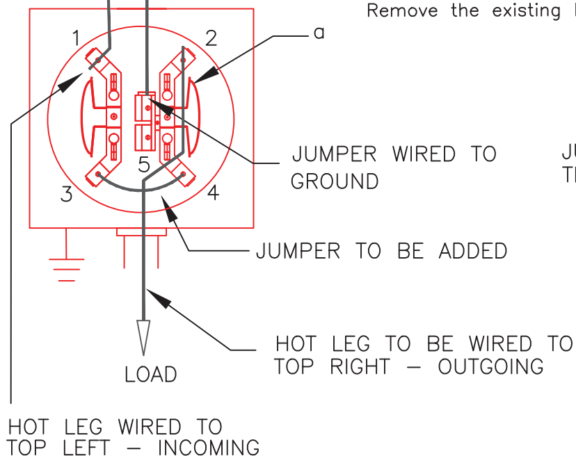
D5S INTERNAL DIAGRAM REAR VIEW
