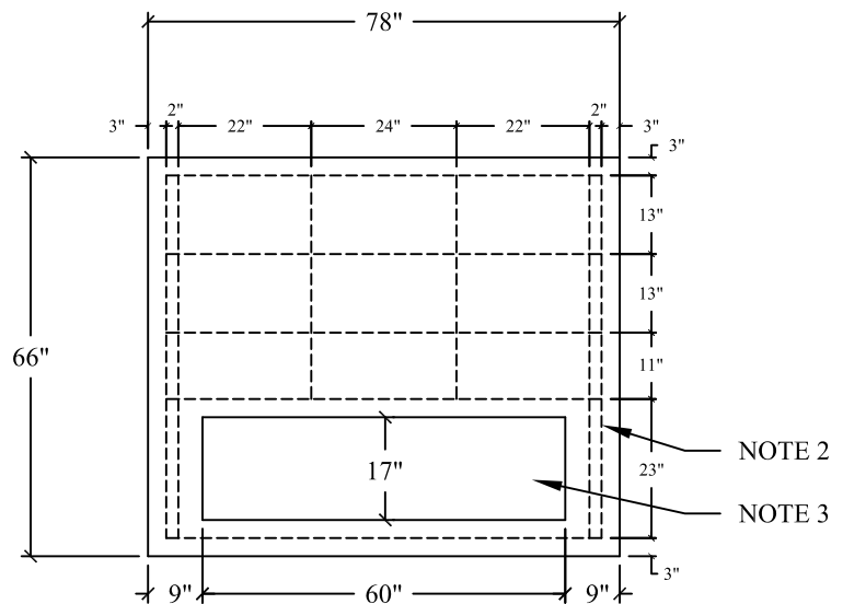
TOP SLAB PLAN VIEW
